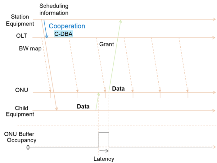
图 3-7 CO-DBA 示例
